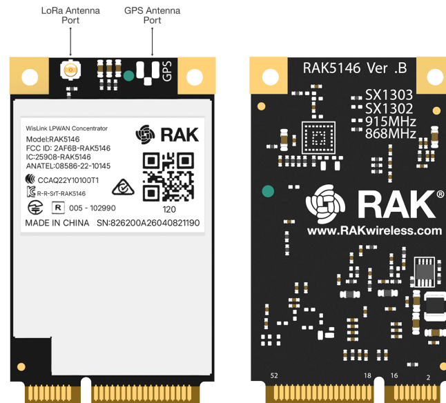
Figure 1: Board Overview
