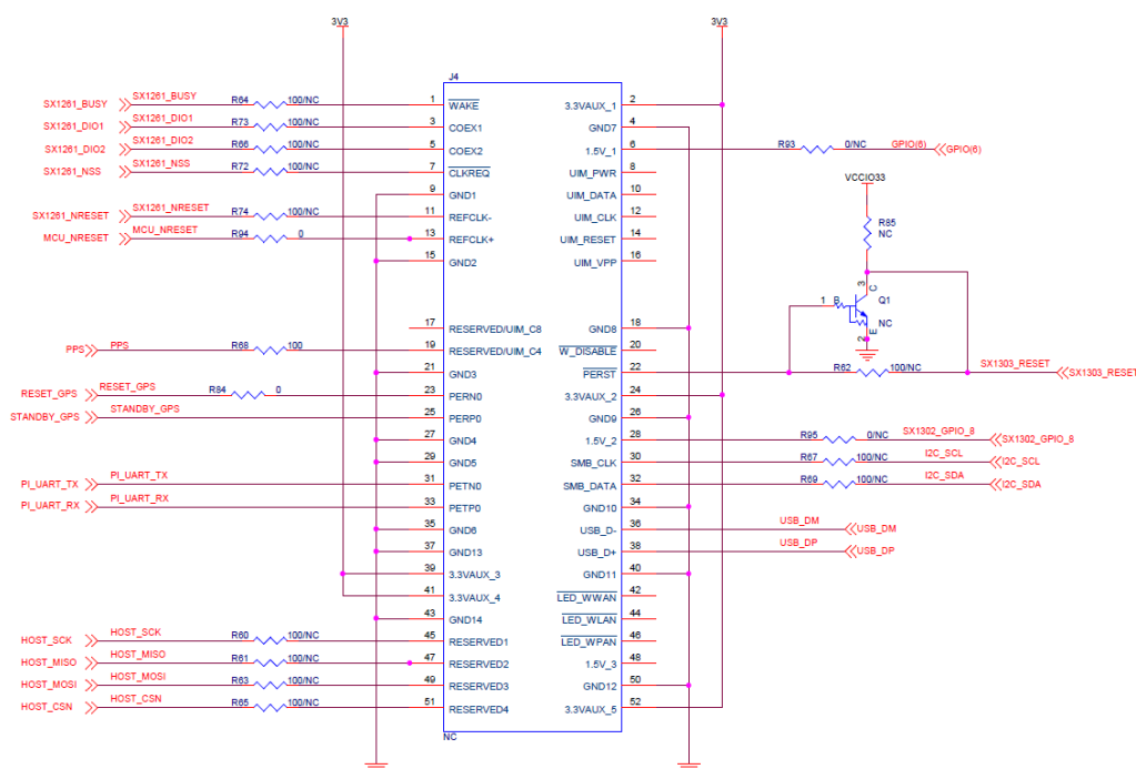
Figure 6: Schematic Diagram
